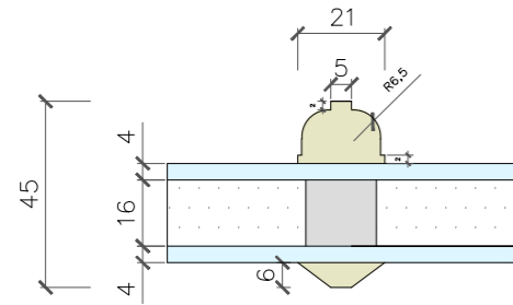
21/5 Bonded Glazing Bar 6.5mm radius Ovolo with Putty Profile Chamfered Bead
