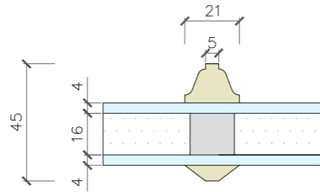
21/5 Lambs (Sash requires 49mm to be fensa spec)
