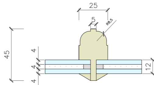
25/5 8.5mm radius Ovolo – Listed building spec
